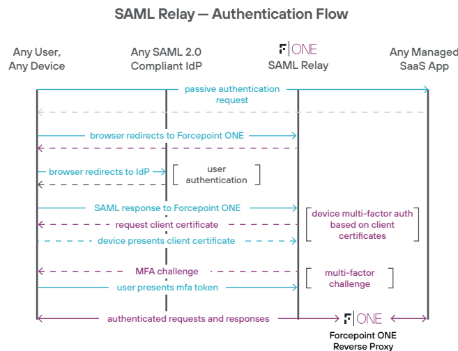
Figure 3: Traffic flow for SAML Relay mode
