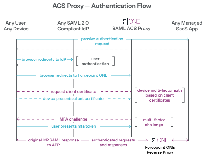
Figure 4: Traffic flow for ACS Proxy mode
